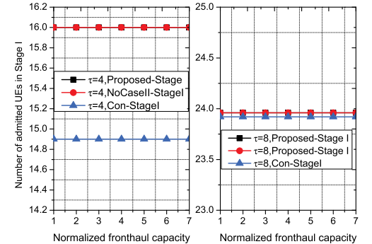
Fig. 13. Number of admitted UEs in Stage I versus the maximum fronthaul capacity \bar{C}_{\max} . The left subplot corresponds to the case of \tau = 4 while the right one is \tau = 8 .
